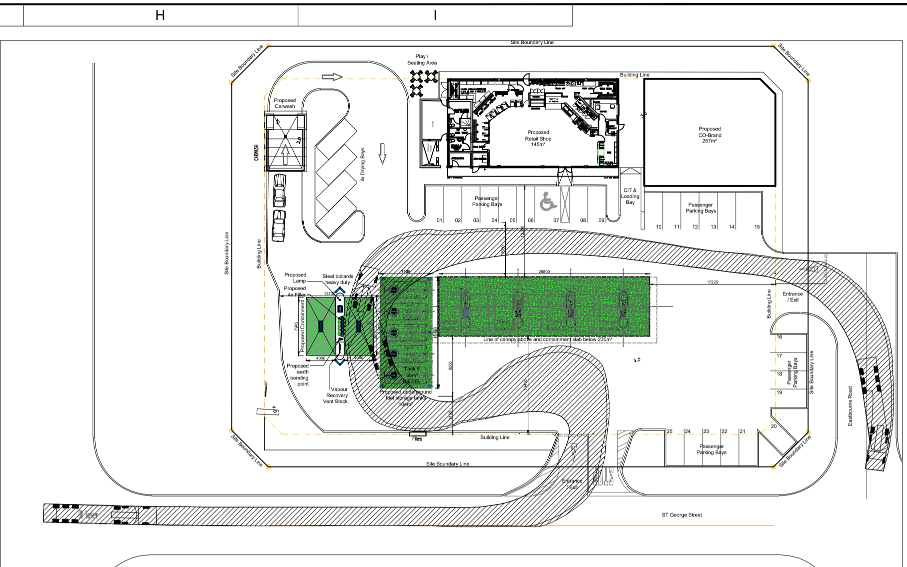
02 Tanker Routing 100 SCALE 1:500
