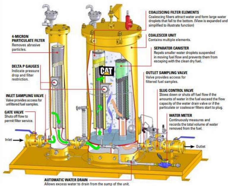
Figure 3: Typical Filter system for Receiving & Bulk Storage Tanks
