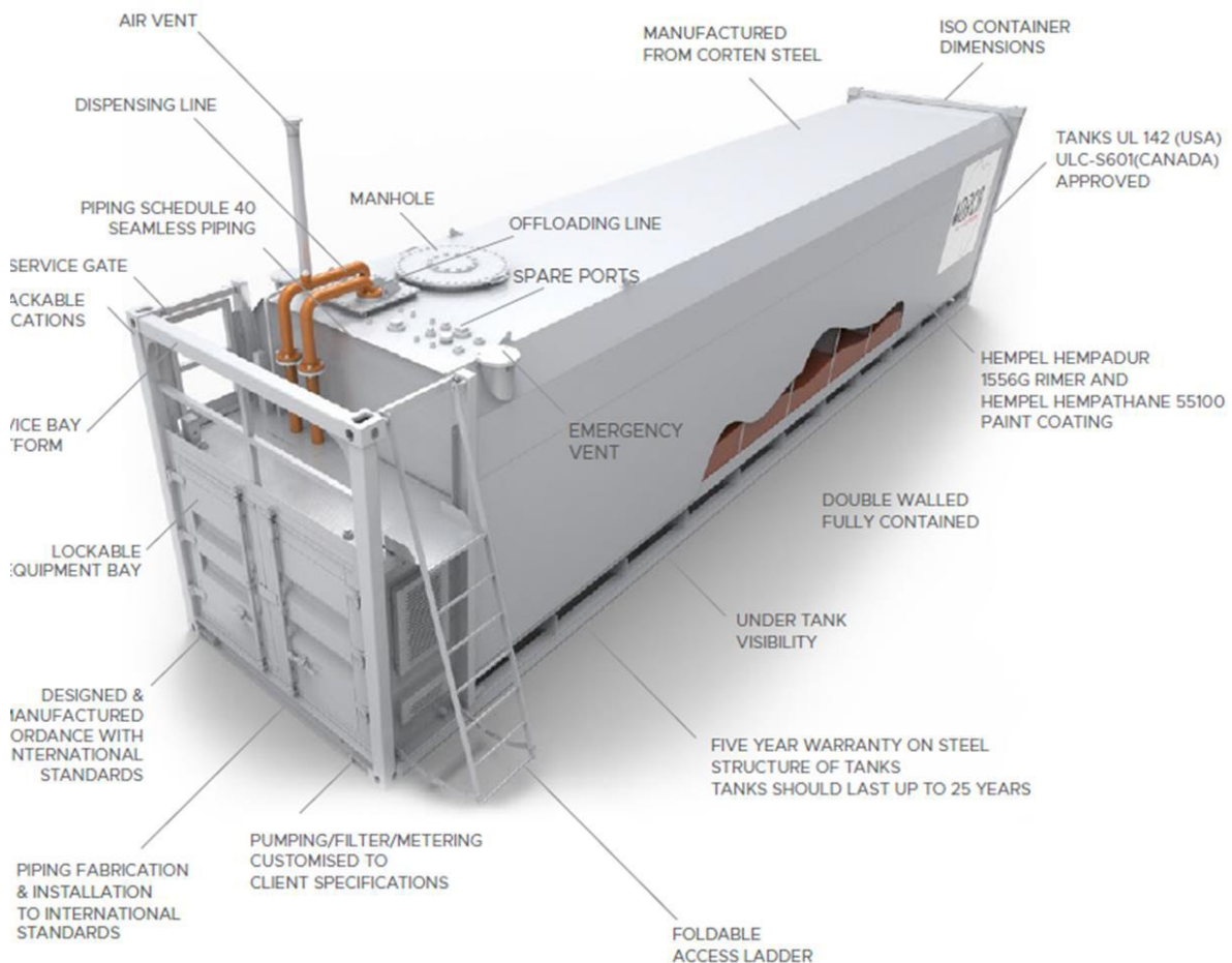
Figure 1: Rendering of proposed containerised fuel farm.
