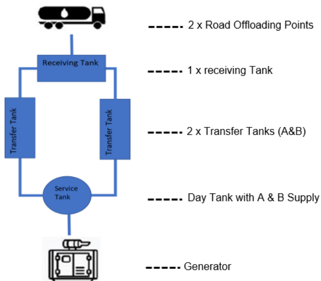
Figure 2: Figure of typical Tier III configuration.
